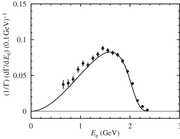
Figure 14.3. The predicted electron-energy spectrum compared with data.
