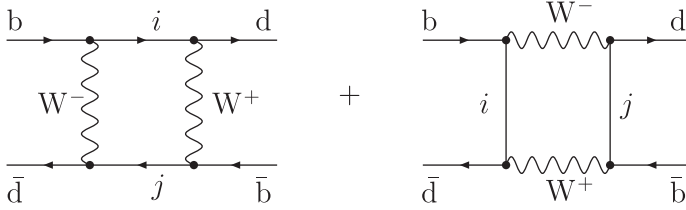
Figure 14.4. Box diagrams for \Delta B = 2 transitions. We calculate the “scattering” term in (a). The “annihilation” term (b) is equal to the “scattering” term.
