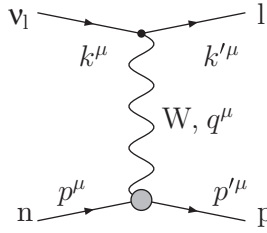
Figure 11.2. Quasi-elastic scattering.
