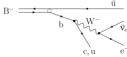
Figure 14.1. B-meson decay.
