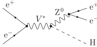
Figure 17.4. Bremsstrahlung from weak bosons.
