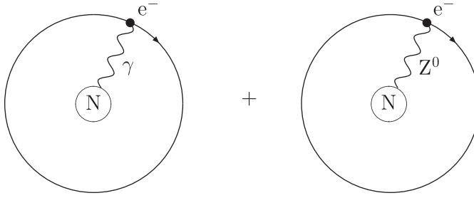
Figure 12.1. A schematic drawing of a Z exchange in an atom.
