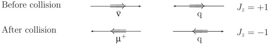
Figure 11.1. Production of a forbidden configuration by helicity conservation in antineutrino–quark scattering.
